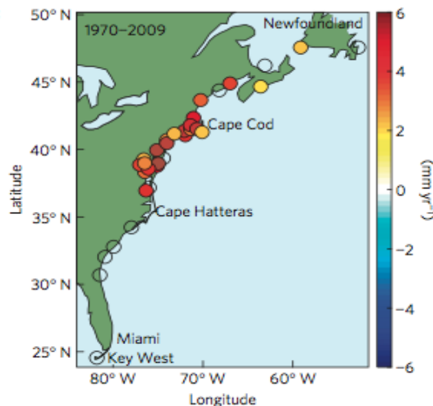
▲ FIGURE 1 Sallenger et al. (2012) identify a 1,000-km stretch of the eastern coast of the United States as a “hotspot” for sea level rise.
