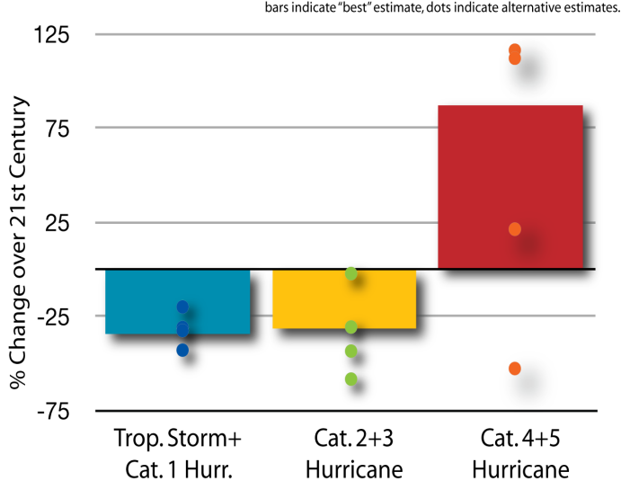
Projected Changes in Atlantic Hurricane Frequency over 21 st Century
