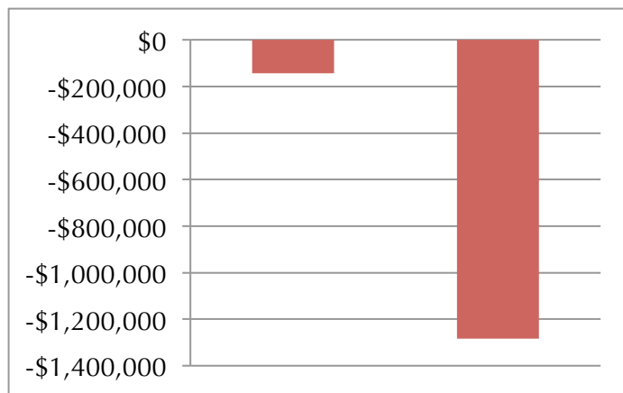
FIGURE 2 Net present values of doing nothing (i.e., no dune) and building a dune with geotextile tubes. Both options cost money, but building a dune would put Stamford much farther “into the red” than would continuing to clean up after storms.
